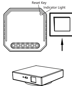
Zigbee Gateway
