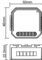
with mounting clip
