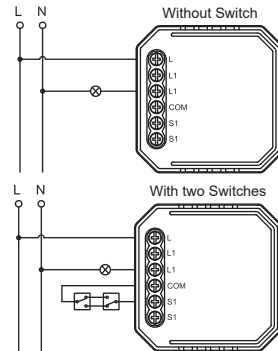
Wiring Instructions and Diagrams
